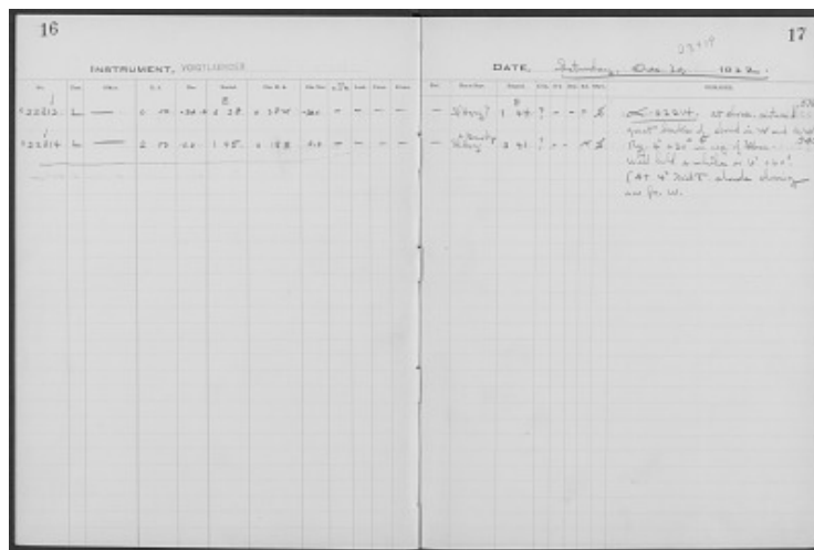
Harvard-Smithsonian Center for Astrophysics DASCH project- Logbook AI #41 Transcribed and Reviewed by Digital Volunteers Extracted Apr-16-2024 12:14:49
